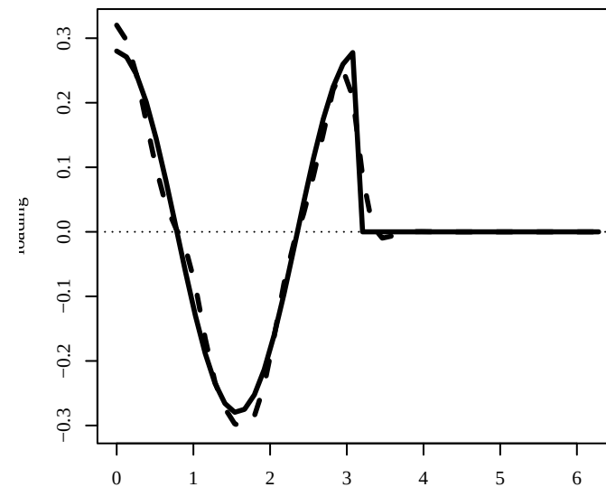
X2 functional piecewise
