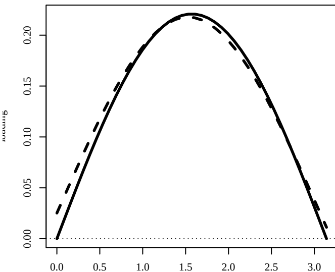
X3 functional smooth
