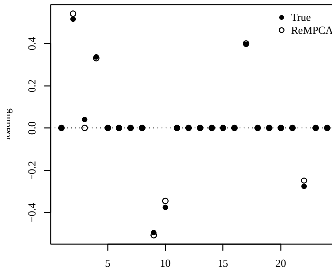
X1 regular sparse
