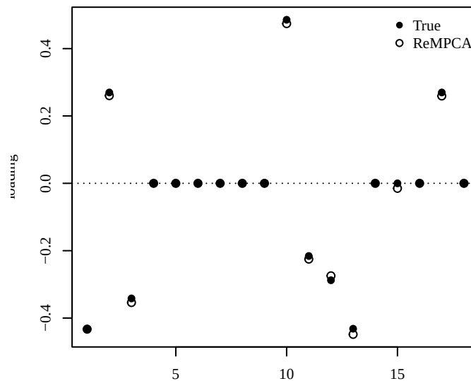
X4 regular block-sparse
