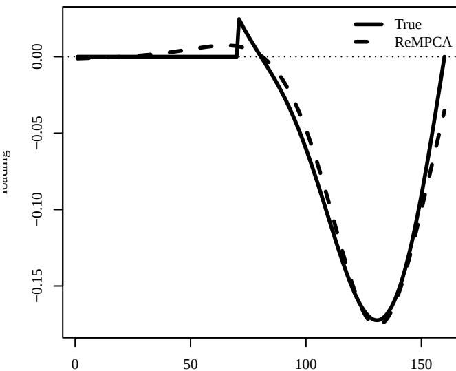
Shared row direction
